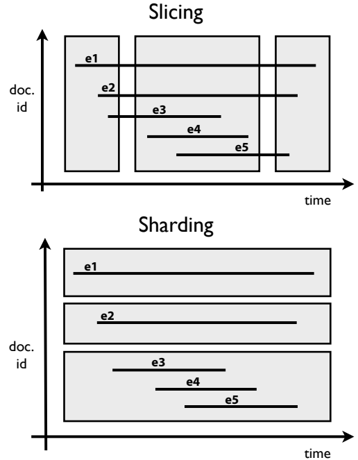
Figure 1: Slicing vs. Sharding of a Index list
