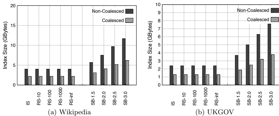
Figure 7: Index sizes
