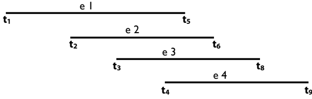
Figure 2: Staircase property
