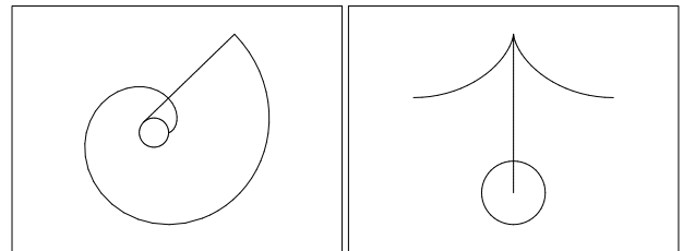
Fig. 13: Left: a circle and its involute. Right: a scheme of Huygens' pendulum with flexible wire and curved metal cheeks.
