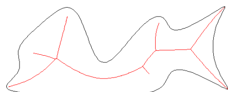
Fig. 18: A closed curve and its skeleton.
