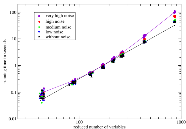
Figure 3: Running times of the Improved-ILP approach to compute one optimal solution.
