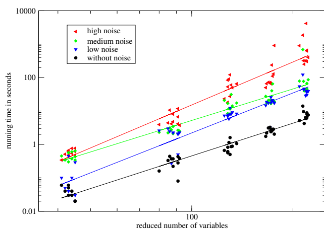
Figure 4: Running times of the improved-ILP approach to enumerate all solutions with minimum error.
