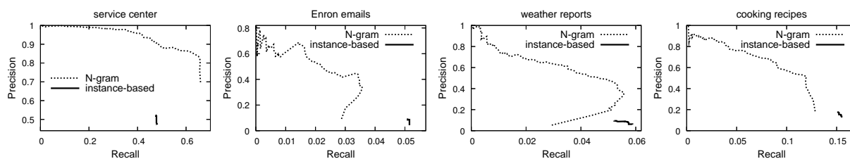
Figure 2: Precision recall curves for N -gram and instance-based methods of sentence completion.
