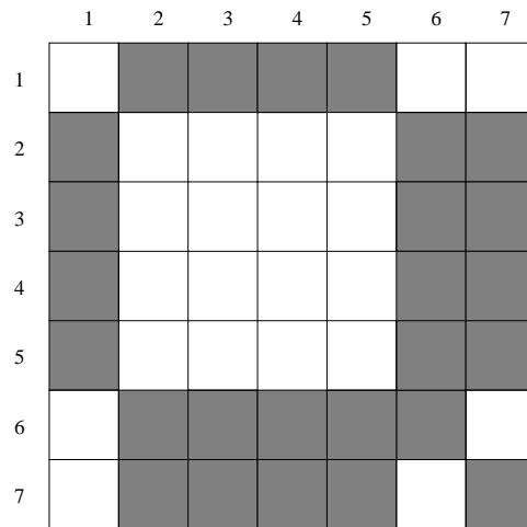
Figure 2: A coloring of \mathcal{G} \times \mathcal{G} with discrepancy 0
