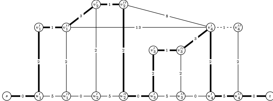
Figure 6: Thick lines are edges of the s - t path consisting of the s - u'_1 line, a u'_1 - u''_2 detour D_1 , the u''_2 - u'_3 line, a u'_3 - u'_4 detour D_2 and the u'_4 - t line. Note that the detour D_1 contains the 1-2 shortcut.
