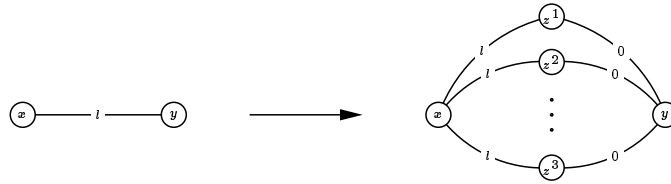
Figure 13: Operation of splitting xy into n copies.
