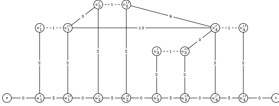
Figure 5: Graph H . Solid lines are fixed edges.
