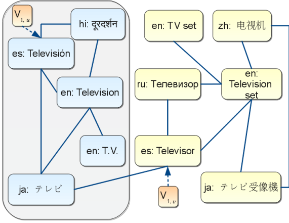
Figure 2: Extended graph with two added nodes v_{1,u} , v_{1,v} representing distinctness between ‘Televi-sión’ and ‘Televisor’, and a region around v_{1,u} that would cut the link from the Japanese ‘Televi-sión’ to ‘Televisor’
