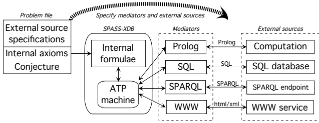
Figure 1: System Architecture
