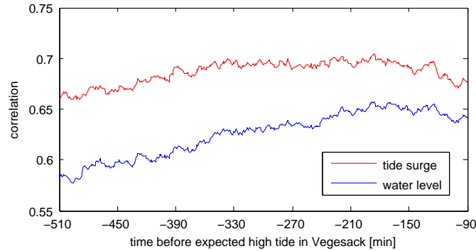
Fig. 3. Correlations between the best projected wind vector with water levels and tide surges.
