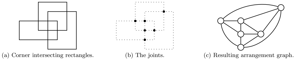
Fig. 2: A set \mathcal{R} of corner intersection rectangles and its arrangement graph A_{\mathcal{R}} .
