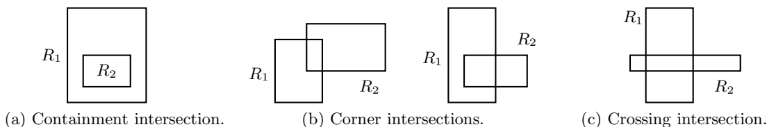
Fig. 1: Possible intersections between two rectangles R_1 and R_2 .
