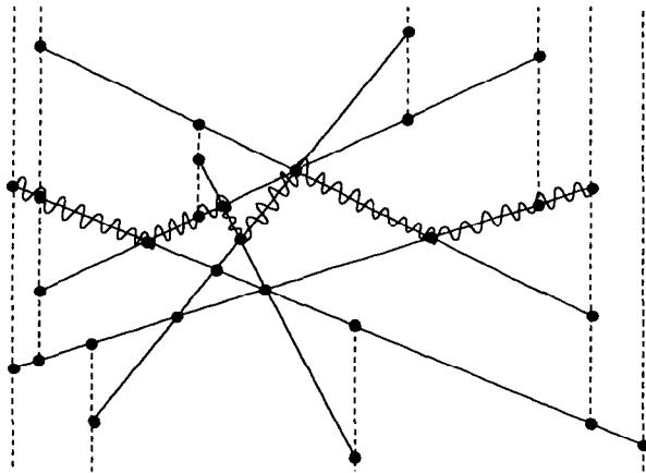
Figure 2: The web graph web(N) . The wiggled line indicates a layer
