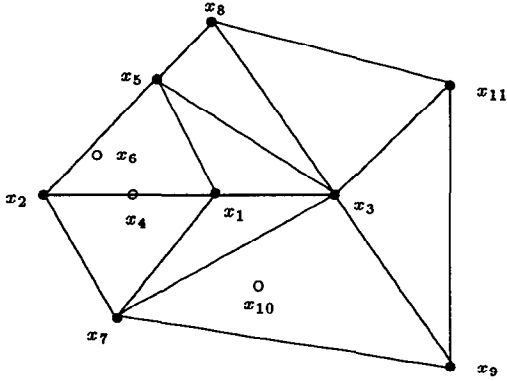
Figure 1: A triangulation. The dimension jumps are points x_1 , x_2 , and x_5 .
