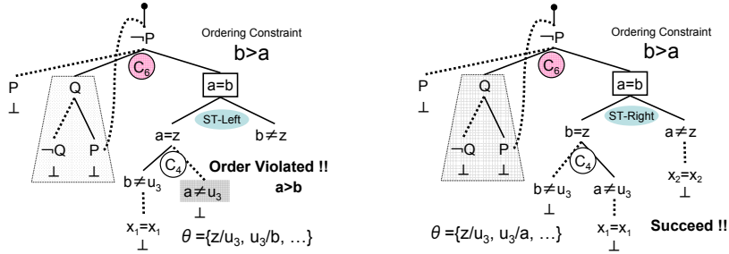
Figure 4: Two connection tableaux in CTwS for nSMT( \mathcal{S}_1 )
