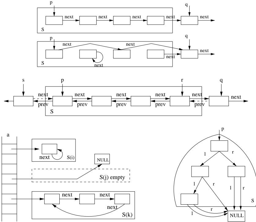
Fig. 3. From top to bottom: shape types S of singly-linked list segments (intended least model and model with unreachable junk), doubly-linked list segments, array of cyclic lists, and binary trees.
