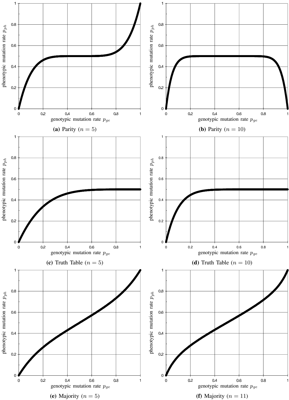
Fig. 1: Mapping from genotypic mutation rate to phenotypic mutation rate for different encodings.
